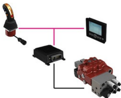
The system is suitable for front loaders (Photo: Walvoil)
