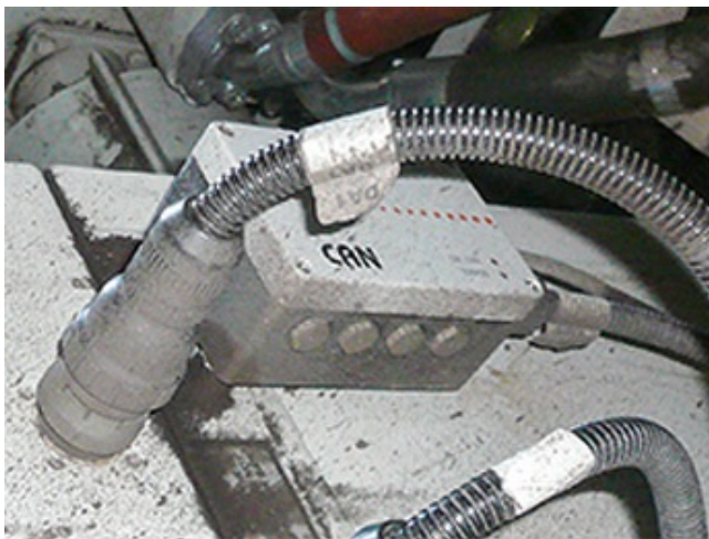
The modules can be installed directly at the signal source e.g. on a dump truck (Source: Microcontrol)
